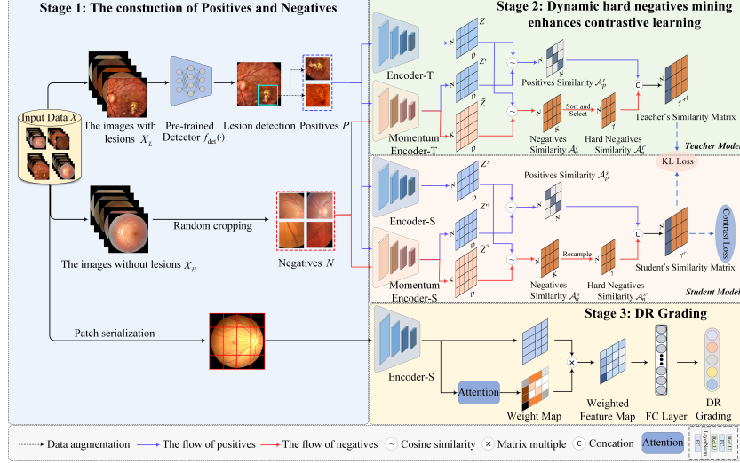
Fig. 1. The overall architecture of the proposed framework. Stage 1: The construction of positives and negatives based on the pre-trained lesion detector. Stage 2: Dynamic hard negatives mining enhances contrastive learning. Stage 3: Fine-tuning our model on the downstream diabetic retinopathy grading task.
