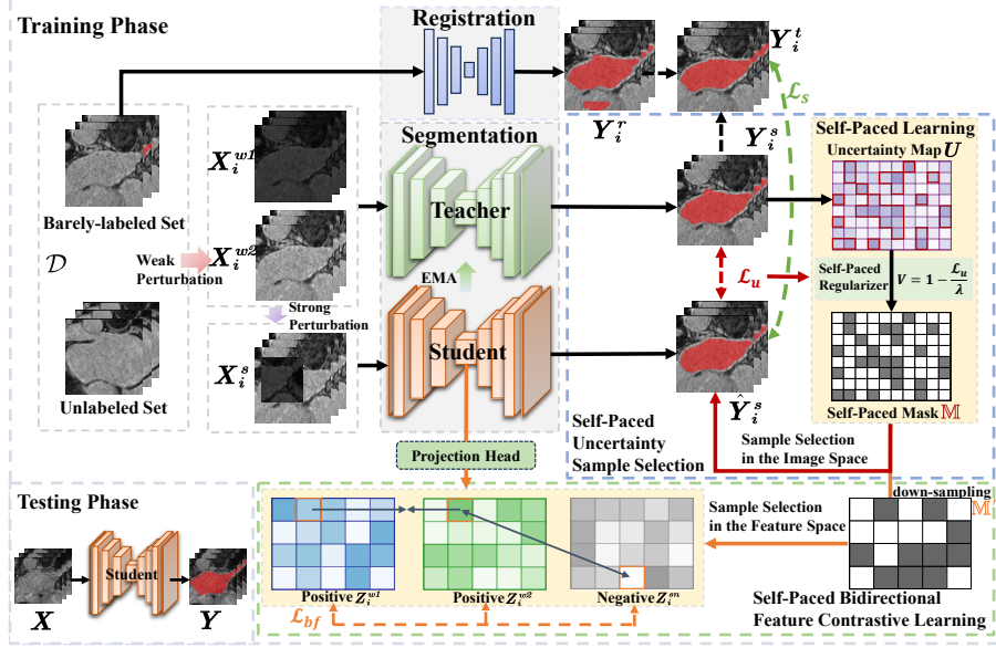
Fig. 2. Overview of the proposed self-paced sample selection framework (SPSS). SPSS includes: 1) a self-paced uncertainty sample selection strategy (SU) for explicitly pseudo labels selection in the image space and 2) a self-paced bidirectional feature contrastive learning scheme (SC) for class semantics discrimination in the feature space.
