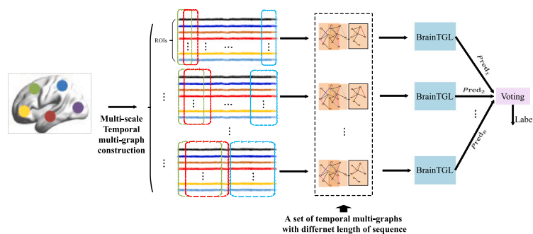
Fig. 7. An ensemble of BrainTGL with multiple window parameters for sliding windows.
