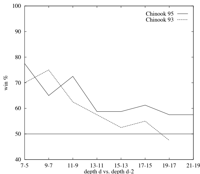
Figure 2: Checkers: Diminishing Returns
