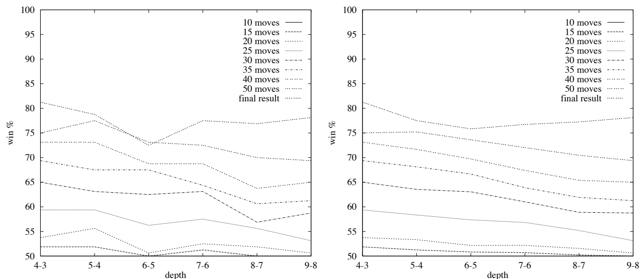
Figure 11: Winning Percentage for Restricted Length Games a) raw b) smoothed
