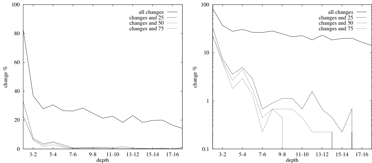
Figure 9: Self-Play Checkers, Move and Value Changes
