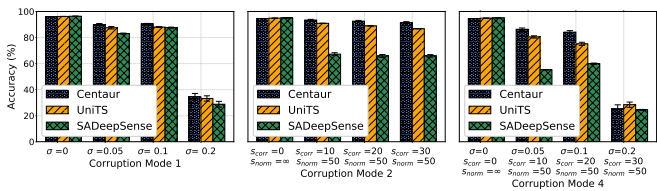
Fig. 6. Performance comparison of Centaur and baseline on HHAR.
