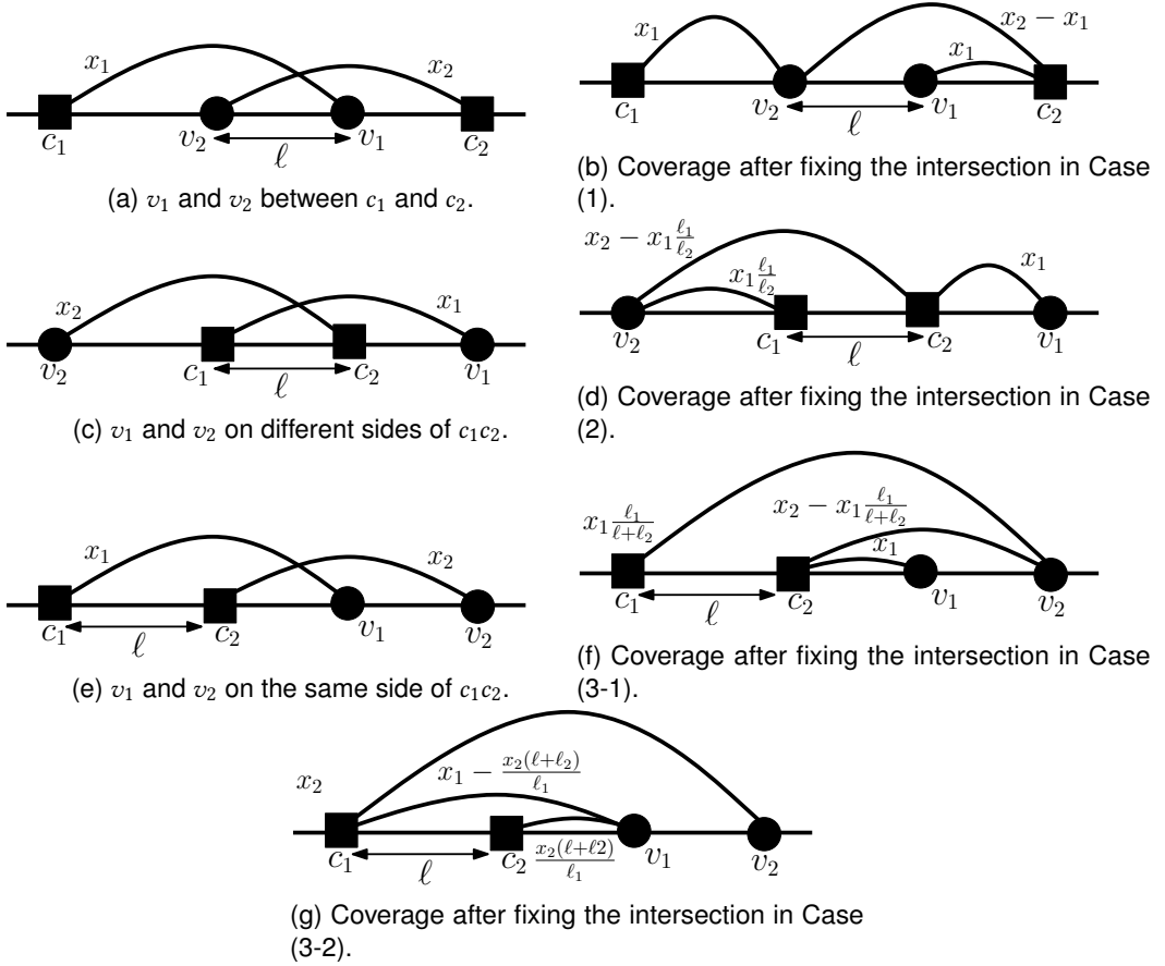
Fig. 1. Fixing the intersection of two small arms.
