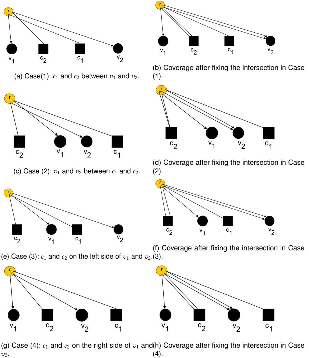
Fig. 4. Fixing the crossing of two arms.
