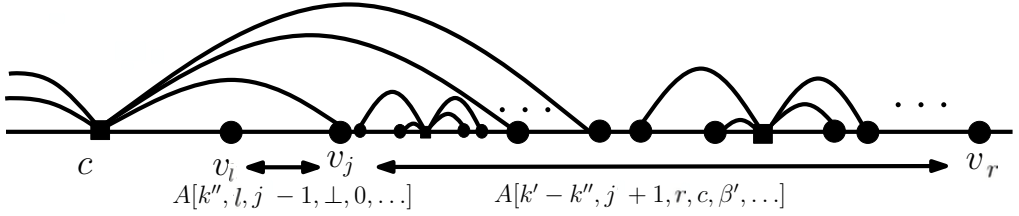
Fig. 2. Case 1 of recursive step
