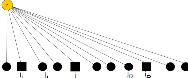
Fig. 5. Moving client assignments. Black solid circles denote clients with x_{ij} > 0 .
