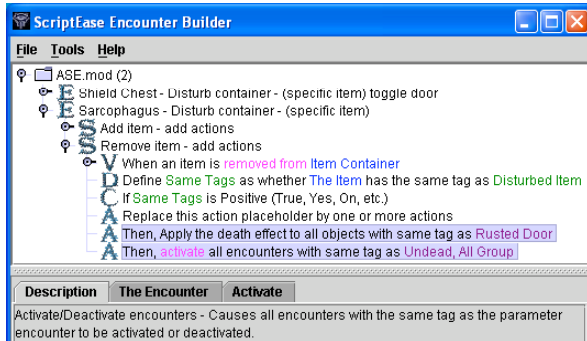
Figure 7. The Encounter Builder.
