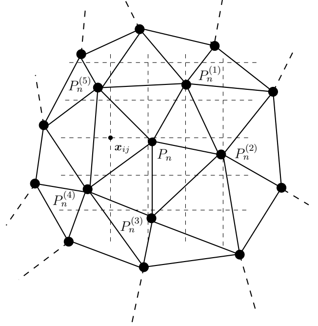
Figure 1. This figure shows a schematic of the non-uniform grid on the rectangular 2D image domain. Here, a section of the grid with a node P_n and its neighboring nodes P_n^{(i)} , i \in \{1, 2, \dots, 5\} is shown. We denote the triangles adjacent to P_n by \delta_{n1} \equiv P_n^{(1)} P_n P_n^{(2)} , \delta_{n2} \equiv P_n^{(2)} P_n P_n^{(3)} ... \delta_{n5} \equiv P_n^{(5)} P_n P_n^{(1)} . The corresponding uniform grid is also shown in dashed lines and a sample pixel \mathbf{x}_{ij} of the uniform grid overlapping with the triangular element of the non-uniform grid is highlighted.
