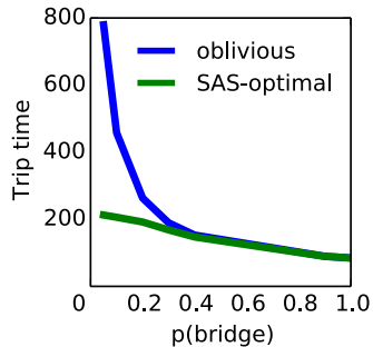
Figure 2: Expected trip time from source to destination under the SAS-optimal policy vs. under the oblivious optimal policy (the MDP solved as if actions are fully available) as a function of bridge availability.
