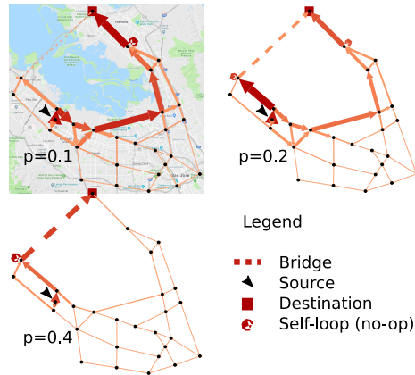
Figure 1: Stochastic action MDPs applied to routing.
