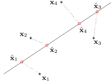
Figure 1. Supervised reverse training attempts to find a linear subspace (determined by the model) in the original data space so that reconstruction of the training examples \mathbf{x}_1, \dots, \mathbf{x}_4 from the targets \mathbf{y}_1, \dots, \mathbf{y}_4 minimizes the sum of squared reconstruction errors.
