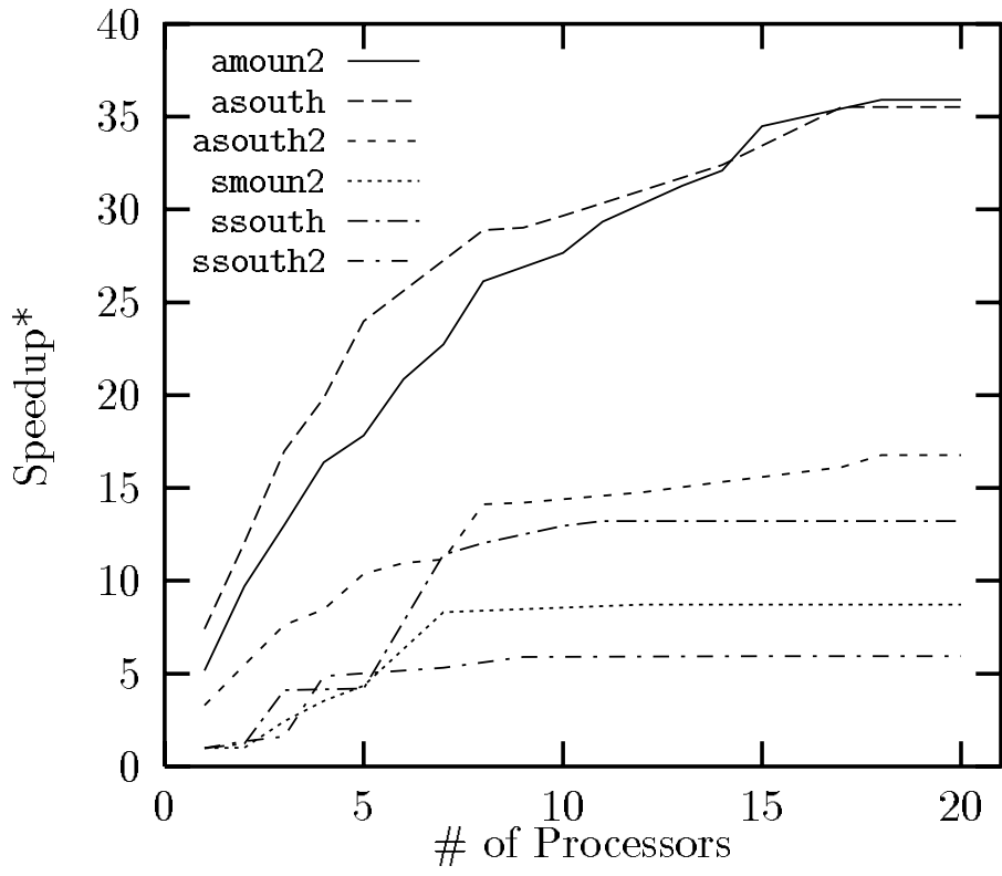
Figure 3: Speedup Curves
