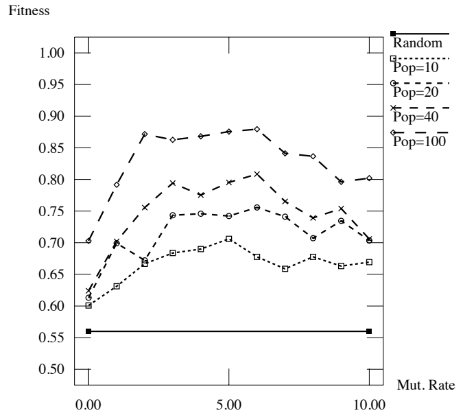
Fig. 1. Effect of the population size on solution quality (40 generations) - c32.
