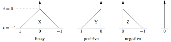
Fig. 5: The four thermographs of loopfree infinitesimals [14, Figure 17].
