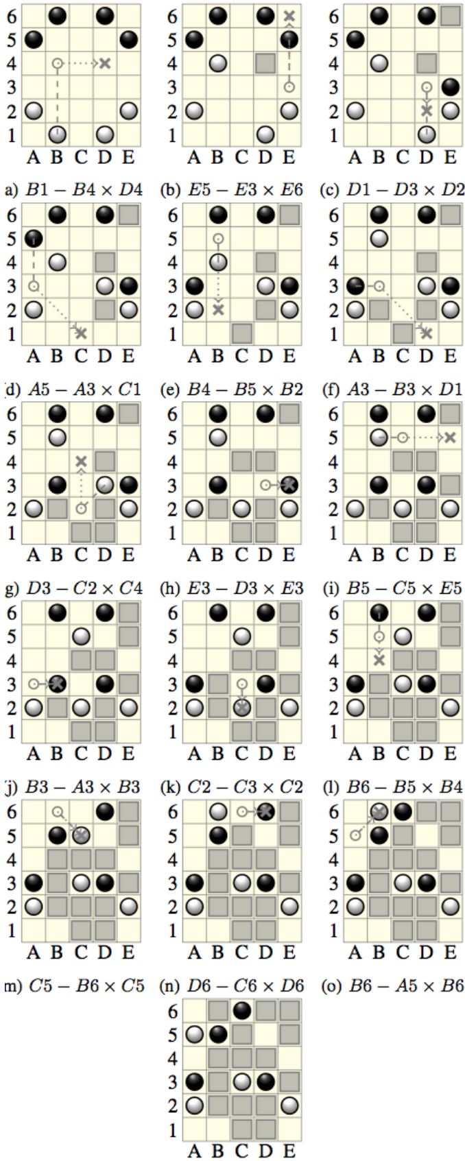
Fig. 14: A sample deep line in the 5 \times 6 proof, White moves first and wins.
