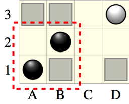
Fig. 9: Blocker territory with 1 normal queen and 1 blocker.
