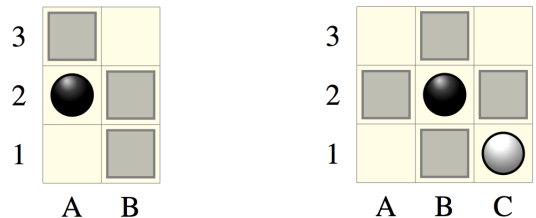
Fig. 7: Territory Bounds: Left: Simple territory, bounds [1, 2] . Right: Blocker territory, bounds [1, 3] .
