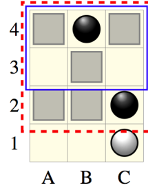
Fig. 10: Territory becomes defective without the blocker C2 .
