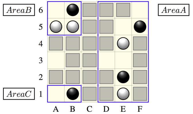
Fig. 12: White to move, global bounds [1 - \epsilon, 3 + \epsilon] .
