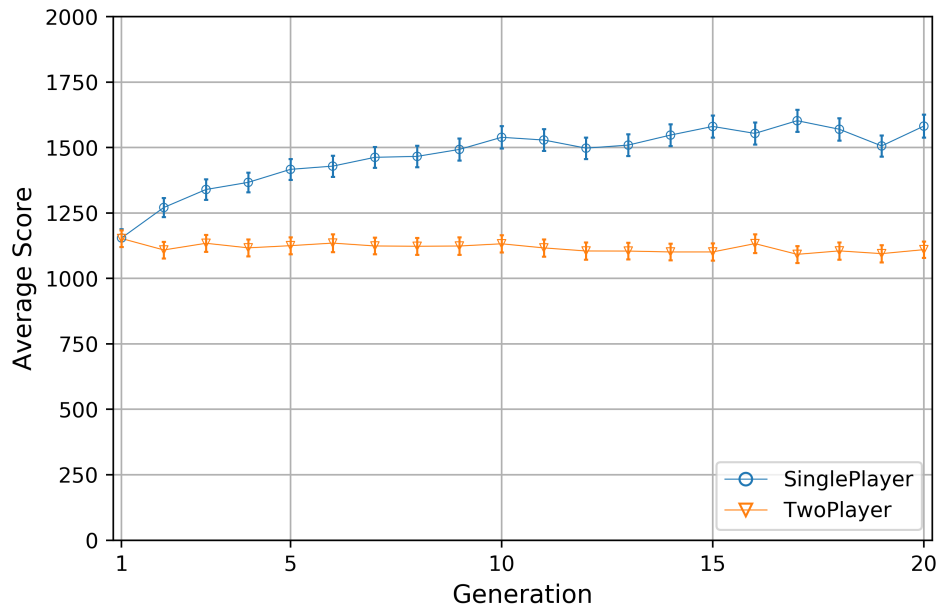
Figure 5.8: Average score of policies during training, for 20 generations, with a single-player or two-player training target.
