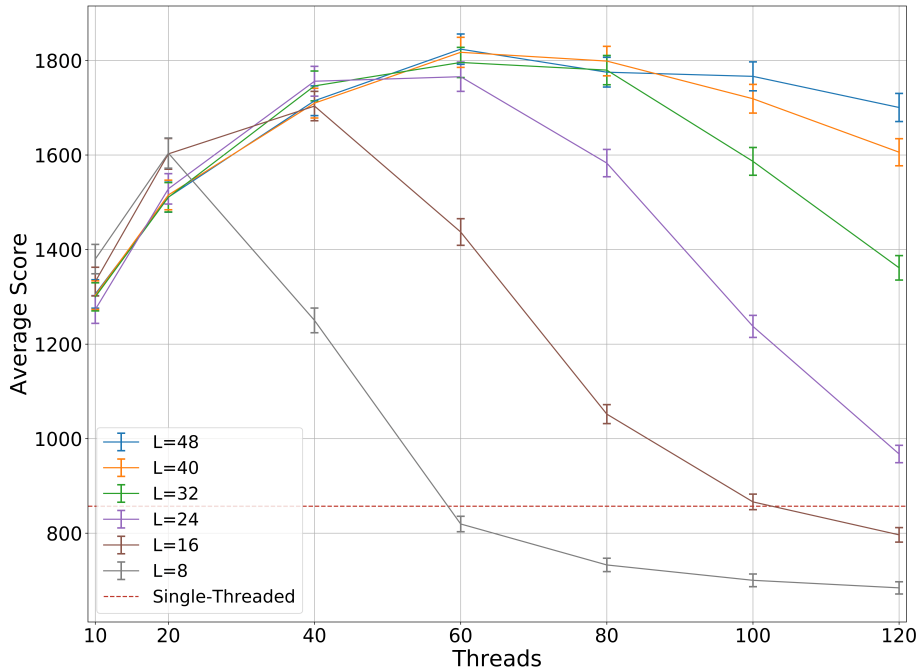
Figure 5.13: The performance of Policy-MCTS, given 1 second of computation time, with different number of threads and queue sizes.
