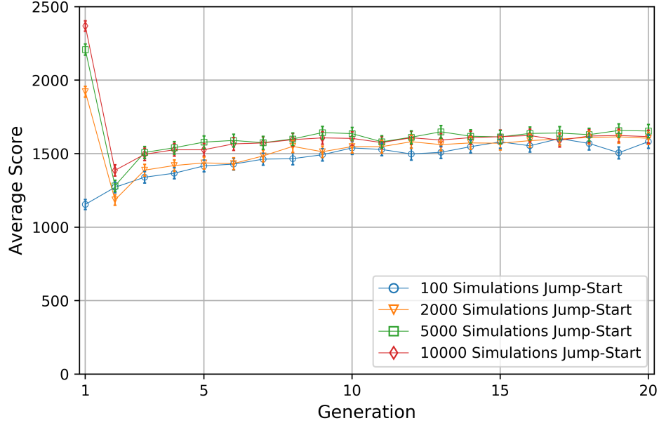
Figure 5.11: Average score of policies during training, for 20 generations, when jump-starting is used. Each policy is trained using a different number of simulations per move in the initial generation.
