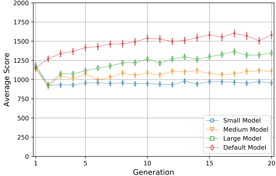
Figure 5.12: Average score of policies during training, for 20 generations, with networks of different sizes.
