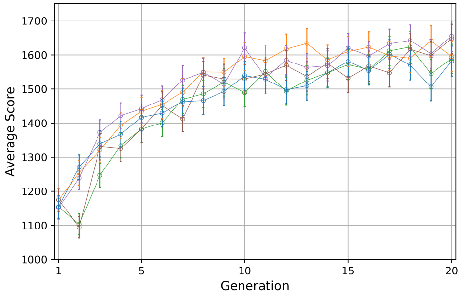
Figure 5.1: Average score of 5 different training runs, all of which use the default parameters provided in Table 5.1.
