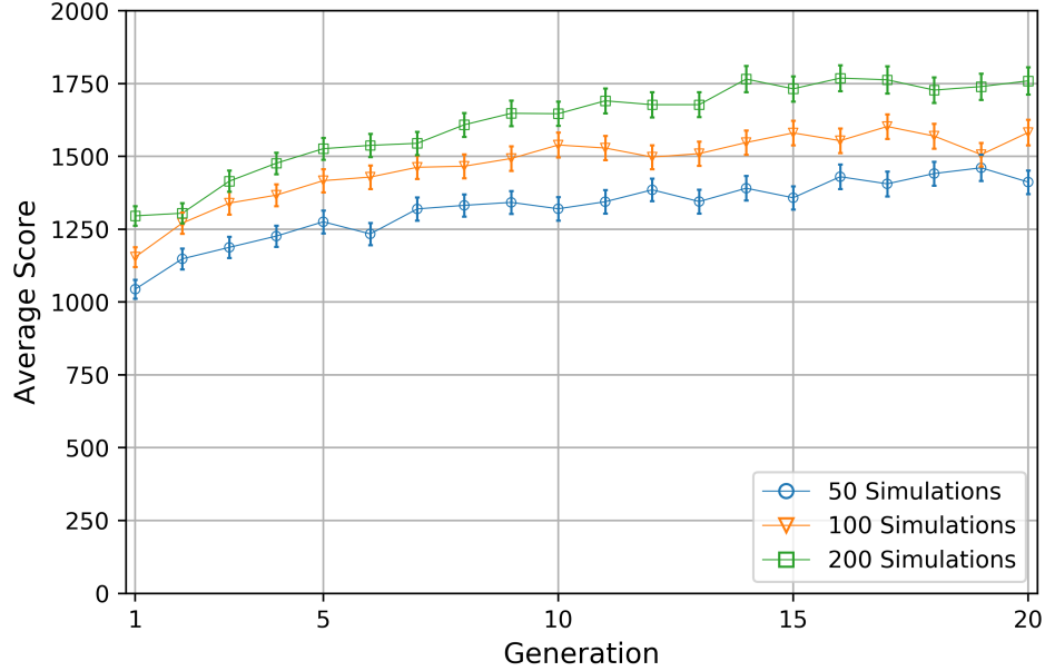
Figure 5.2: Average score of policies during training, for 20 generations, with varying number of simulations per move.
