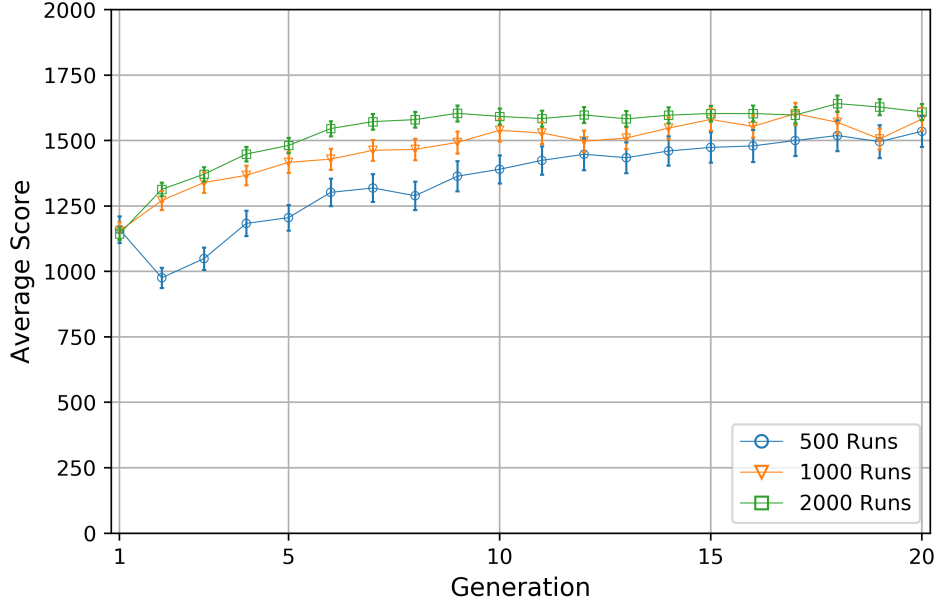
Figure 5.4: Average score of policies during training, for 20 generations, with varying number of runs per generation.
