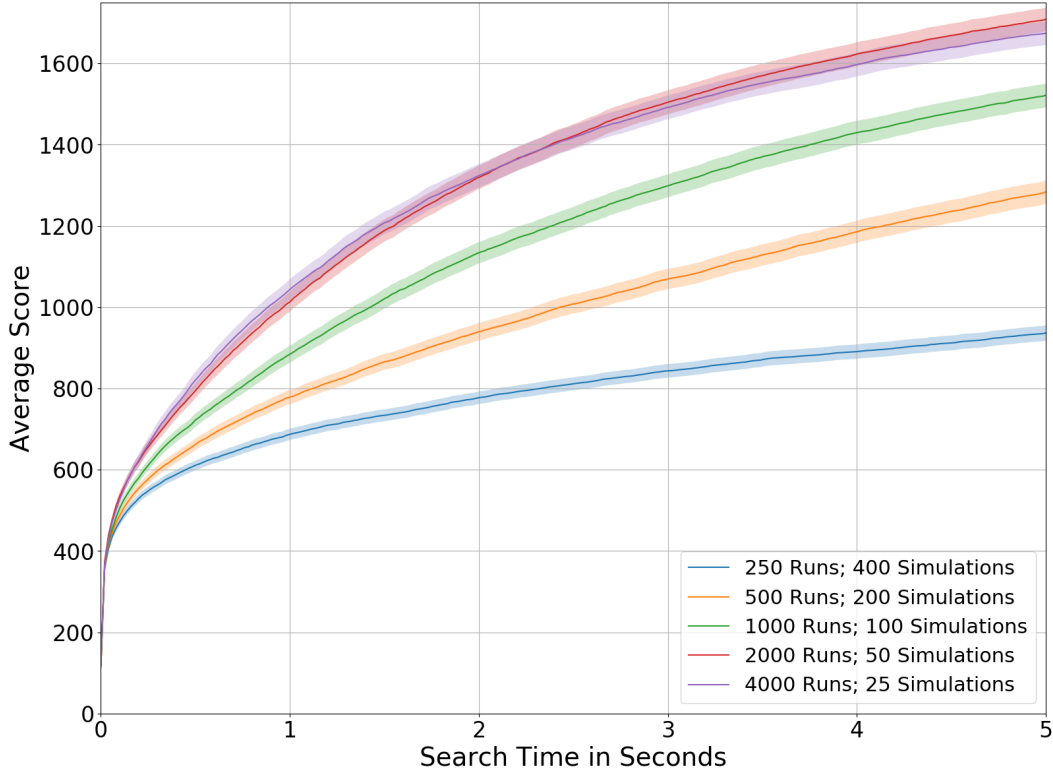
Figure 5.7: Comparing the performance of policies trained for 5 hours, with varying number of runs per generation and simulations per move. The y-axis depicts the average score attained on 500 boards, with 5 runs on each, for a total of 2,500 runs. Each run is given up to 5 seconds of computation time per run, indicated by the x-axis. The shaded areas indicate the 99% confidence bands.
