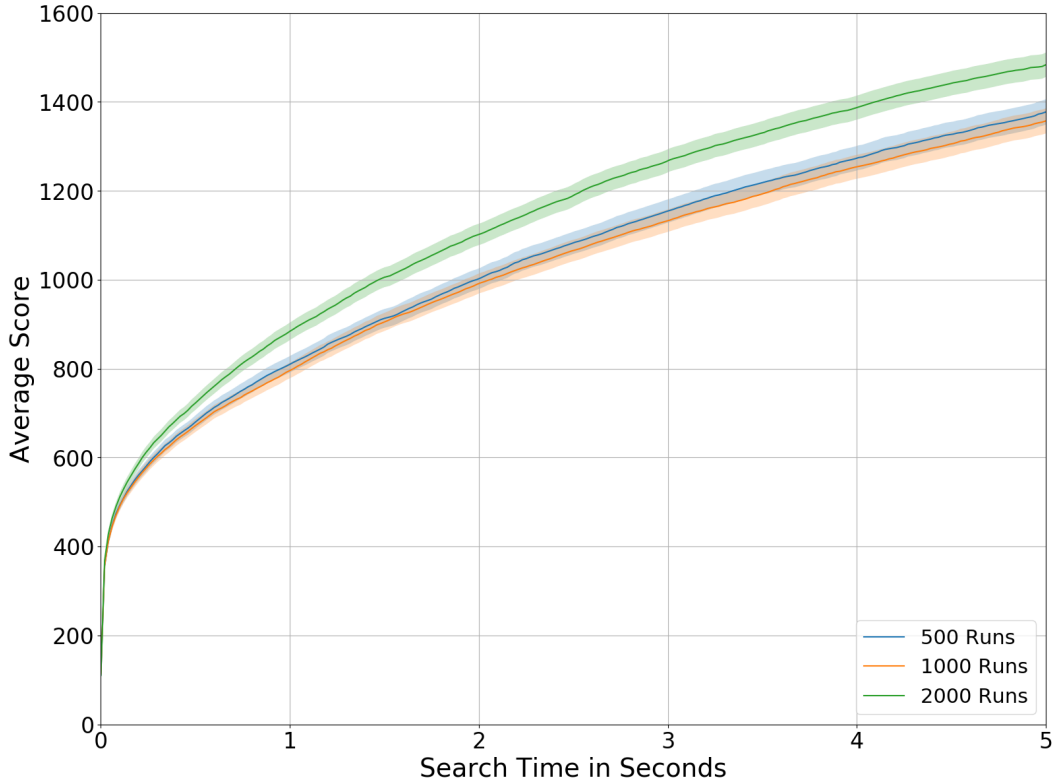
Figure 5.5: Comparing the performance of Policy-MCTS using policies trained for 20 generations, with varying number of runs per generation. The y-axis depicts the average score attained on 500 boards, with 5 runs on each, for a total of 2,500 runs. Each run is given up to 5 seconds of computation time per run, indicated by the x-axis. The shaded areas indicate the 99% confidence bands.
