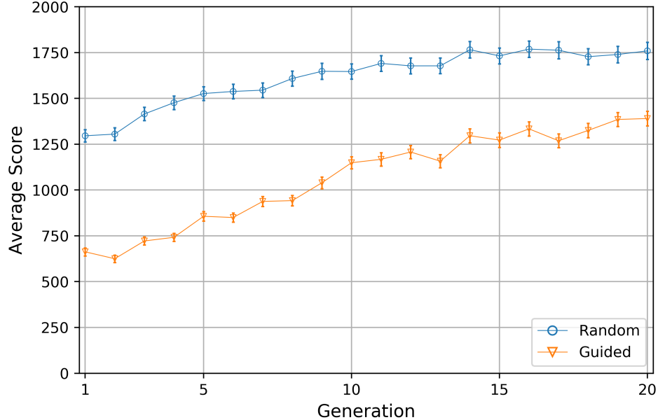
Figure 5.9: Average score of policies during training, for 20 generations, with 5 guided or 200 random rollouts.
