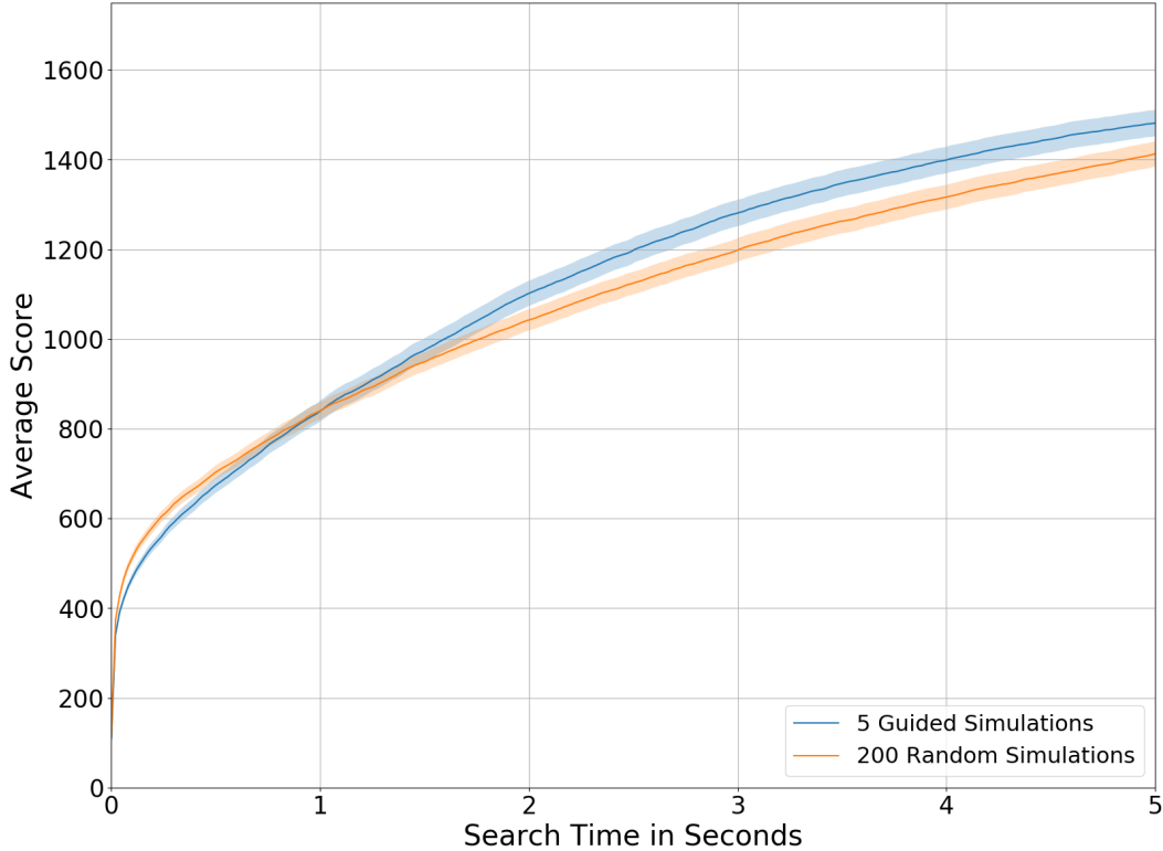
Figure 5.10: Comparing the performance of Policy-MCTS using policies trained for 20 generations, with random, or guided rollouts, respectively. The y-axis depicts the average score attained on 500 boards, with 5 runs on each, for a total of 2,500 runs. Each run is given up to 5 seconds of computation time per run, indicated by the x-axis. The shaded areas indicate the 99% confidence bands.
