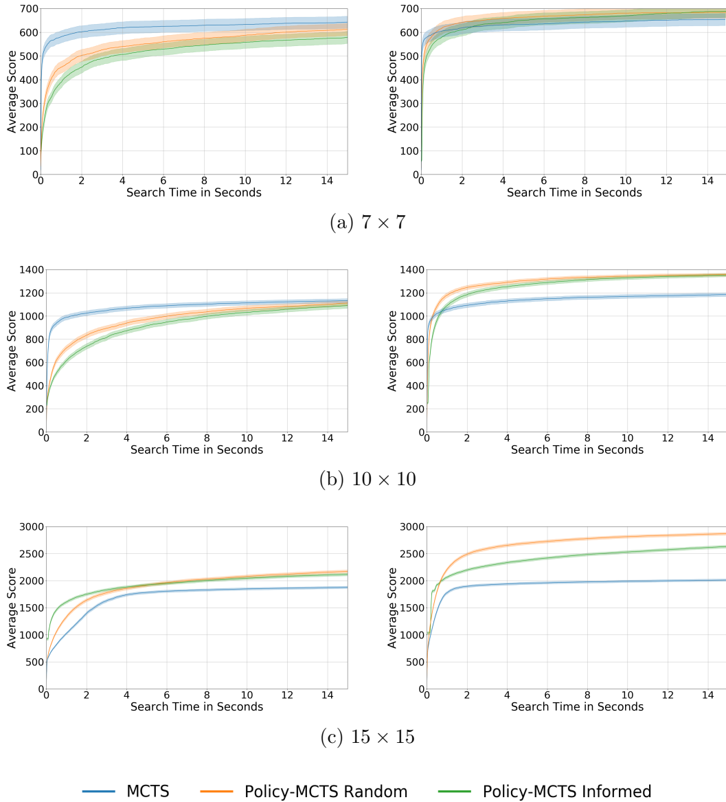
Figure 5.16: Average score of single-threaded (left) and multi-threaded (right) MCTS, Policy-MCTS with random rollouts, and Policy-MCTS with informed rollouts, as a function of search time in seconds. All policies are trained using informed rollouts. Each experiment is performed on a test set of 500 randomly generated boards, with 5 runs per board. The shaded areas indicate the 99% confidence bands.
