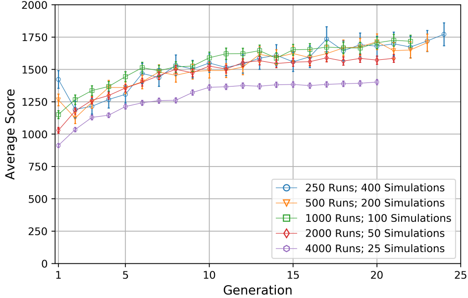
Figure 5.6: Average score of policies during training, given a total time limit of 5 hours, with varying number of runs per generation and simulations per move.
