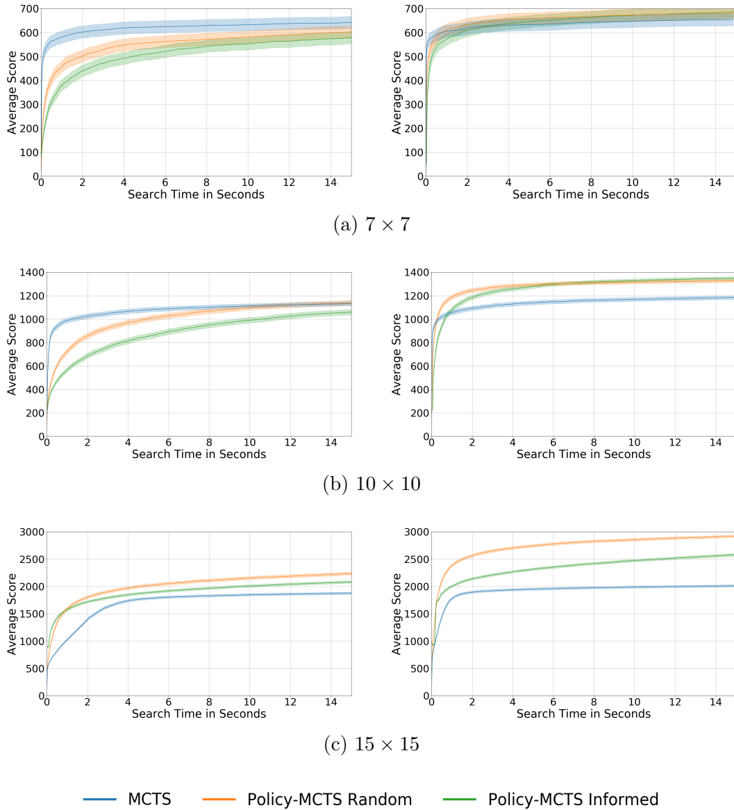
Figure 5.15: Average score of single-threaded (left) and multi-threaded (right) MCTS, Policy-MCTS with random rollouts, and Policy-MCTS with informed rollouts, as a function of search time in seconds. All policies are trained using random rollouts. Each experiment is performed on a test set of 500 randomly generated boards, with 5 runs per board. The shaded areas indicate the 99% confidence bands.
