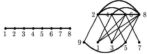
Figure 5: A non-extending prime non-degenerate subrealization of a realizable hypergraph. The graph G' on the left is a subrealization of the P_4 -structure H of the graph G on the right. G' does not extend to any realization of H , because G is strongly uniquely realizable (since G[\{v_1, \dots, v_5, v_9\}] is isomorphic to the graph in Figure 1).
