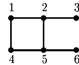
Figure 1: A realization of a strongly uniquely realizable hypergraph.
