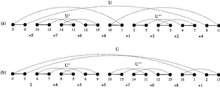
FIG. 4. (a) Unoriented component U separates U' and U'' by virtue of the edge (0, 1) ; (b) Hurdle U does not separates U' and U'' .
