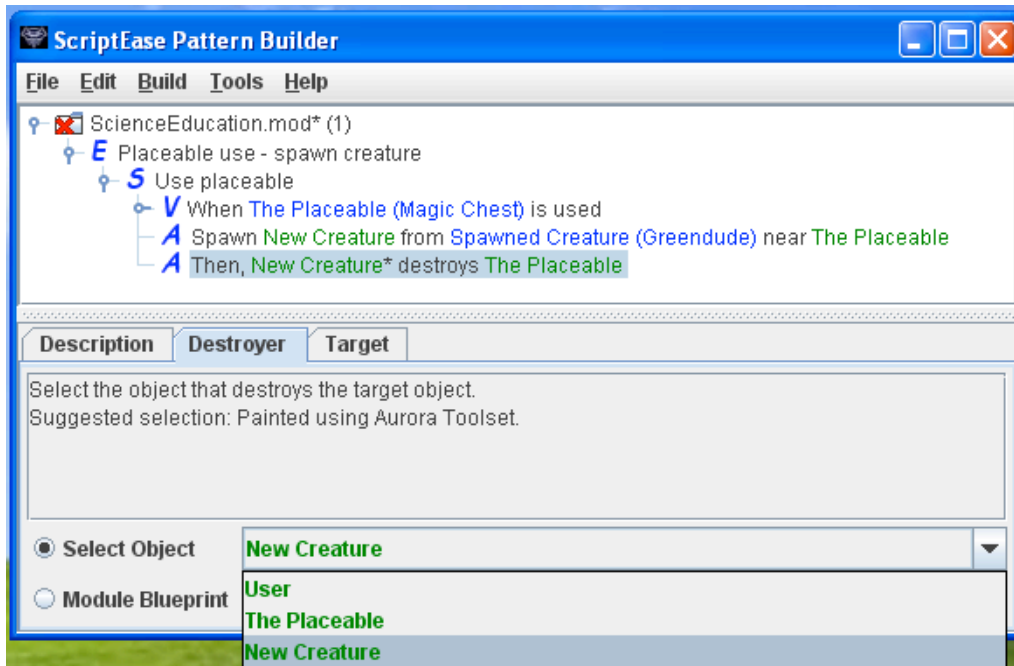
Figure 4. Adding an action to a pattern and setting its options.
