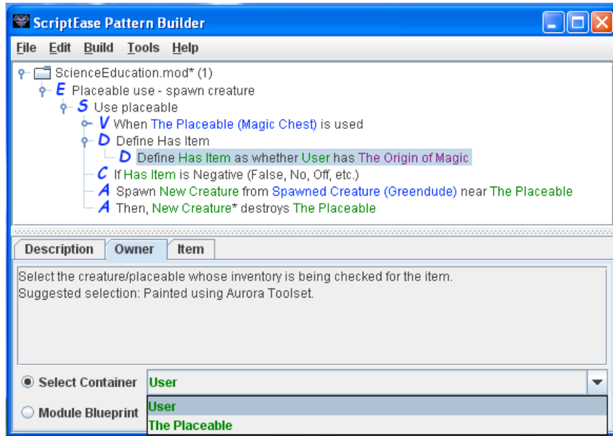
Figure 6. Adding a definition and condition to a pattern and setting their options.
