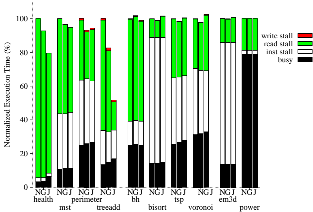
Figure 6. Prefetching performance
