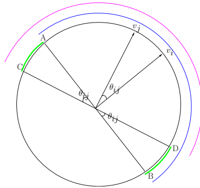
Figure 17.1: The vector \vec{r} will separate v_i and v_j , if it falls in one of the green arcs AC or BD
