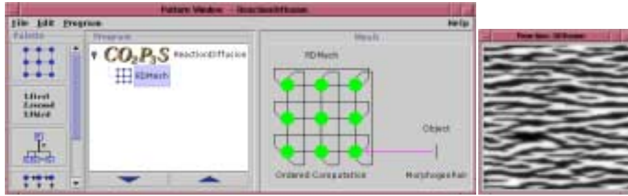
(a) A screenshot of the Mesh template in \text{CO}_2\text{P}_3\text{S} . (b) Output image.
