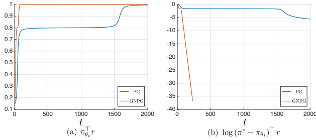
Figure 4. PG and GNPG on r = (1.0, 0.8, 0.1)^\top .
