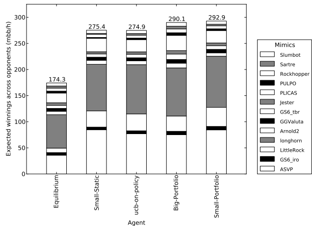
Figure 4: Performance versus mimics corresponding to the responses in the large portfolio. Bar components are in the same order as the legend.
