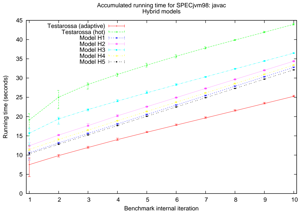
Figure A.12: Hybrid models on javac.
