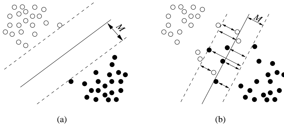
Figure 3.1: Example of hyperplane placement. When the data is linearly separable (a), the separating hyperplane (solid line) is placed as far as possible from either class (hollow and filled circles) with a margin of M , and the support vectors (dashed lines) lie at the instances closest to the hyperplane, from both classes. When the data is overlapping (b), some amount of misclassification must be allowed (arrows) during hyperplane placement.
